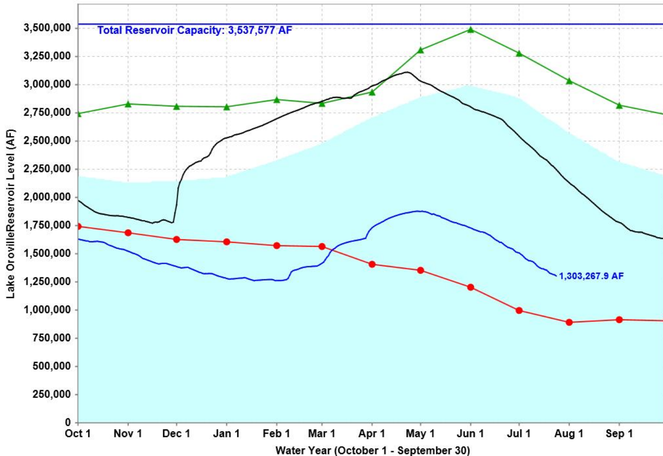
Lake Oroville Levels: Various Past Water Years and Current Water Year, Ending At Midnight July 24, 2014
