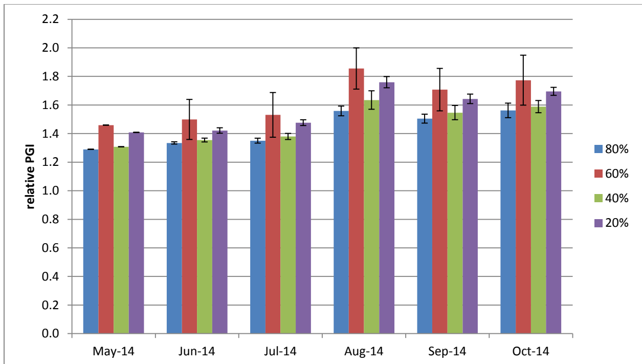
Figure 15b. Average monthly relative plant growth index of Buddleia ‘Purple Splendor’ in 2014 on 4 ET_0 -based irrigation levels. Bars represent \pm 1 SE. There were no significant differences using ANOVA and Tukey’s HSD at p < 0.05 .
