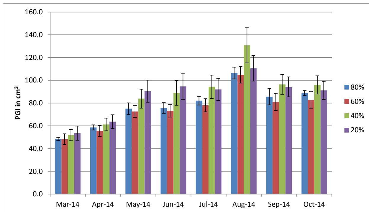
Figure 25a. Average monthly plant growth index of Lonicera 'Peaches and Cream' in 2014 on 4 ET_0 -based irrigation levels. Bars represent \pm 1 SE. No significant differences using ANOVA and Tukey's HSD at p < 0.05 .
