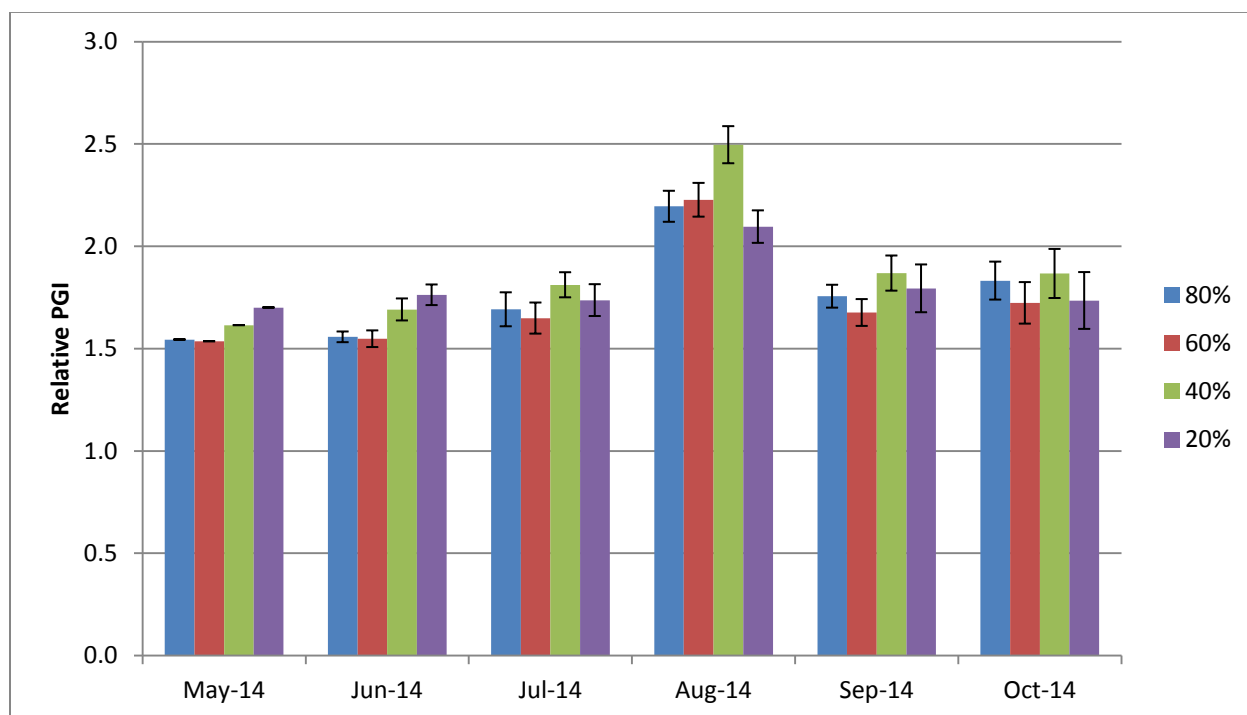
Figure 25b. Average relative monthly plant growth index of Lonicera 'Peaches and Cream' in 2014 on 4 ET_0 -based irrigation levels. Bars represent \pm 1 SE. No significant differences using ANOVA and Tukey's HSD at p < 0.05 .
