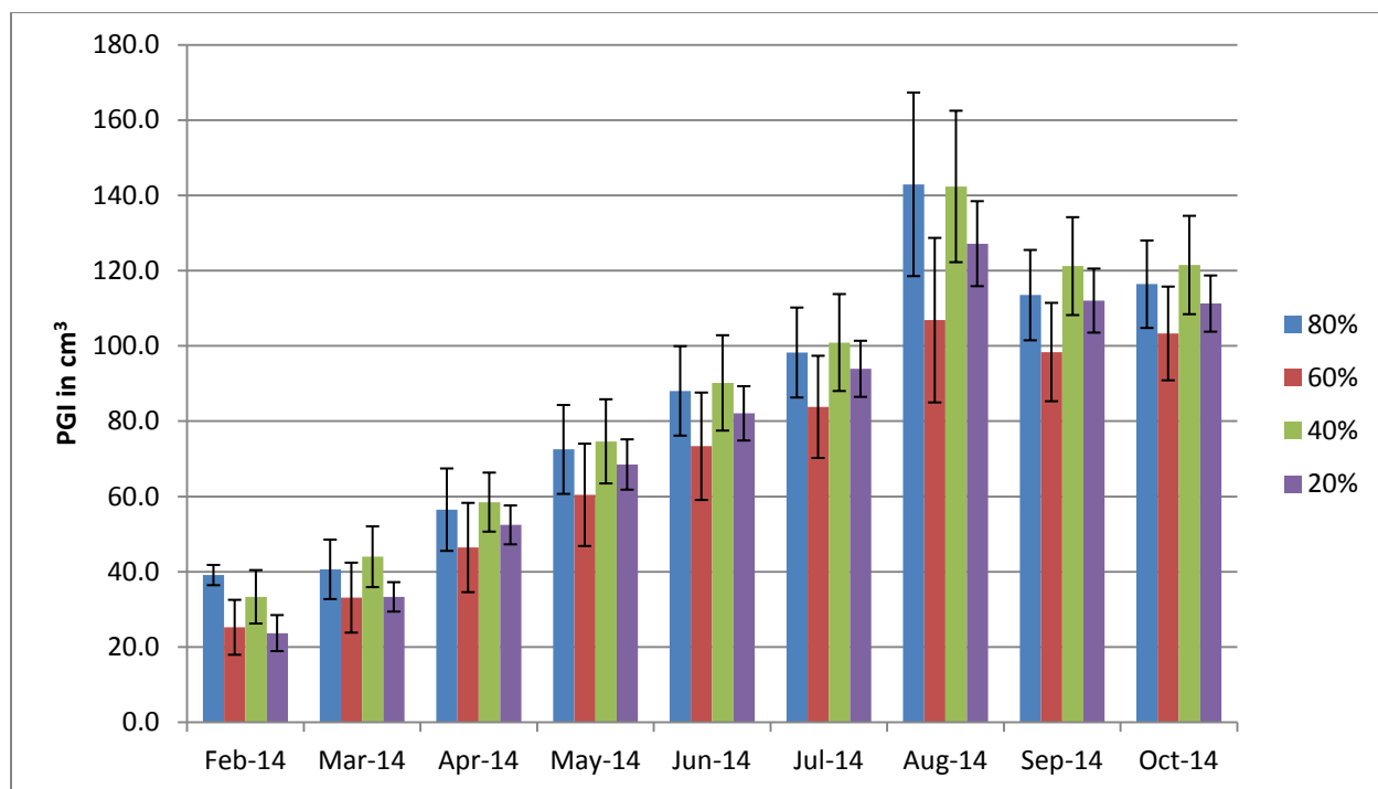
Figure 19a. Average monthly plant growth index of Epilobium 'Sierra Salmon' in 2014 on 4 \text{ET}_0 -based irrigation levels. Bars represent \pm 1 SE. There were no significant differences using ANOVA and Tukey's HSD at p < 0.05 .
