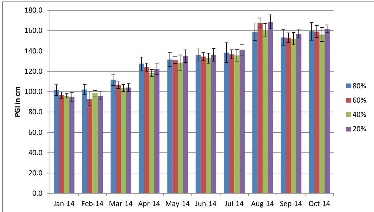
Figure 15a. Average monthly plant growth index of Buddleia ‘Purple Splendor’ in 2014 on 4 ET_0 -based irrigation levels. Bars represent \pm 1 SE. There were no significant differences using ANOVA and Tukey’s HSD at p < 0.05 .
