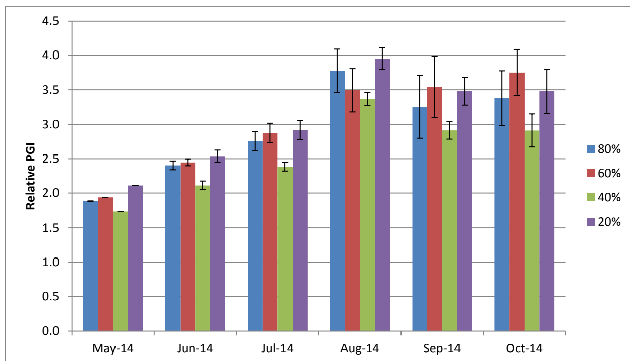
Figure 19b. Average monthly relative plant growth index of Epilobium 'Sidewinder' in 2014 on 4 \text{ET}_0 -based irrigation levels. Bars represent \pm 1 SE. There were no significant differences using ANOVA and Tukey's HSD at p < 0.05 .
