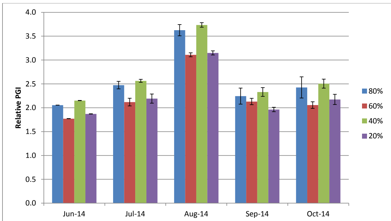
Figure 18b. Average monthly relative plant growth index of Epilobium 'Sidewinder' in 2014 on 4 ET_0 -based irrigation levels. Bars represent \pm 1 SE. There were no significant differences using ANOVA and Tukey's HSD at p < 0.05 .
