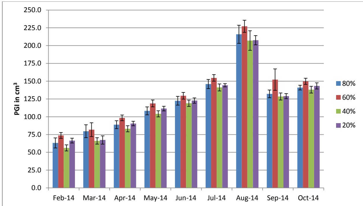
Figure 18a. Average monthly plant growth index of Epilobium 'Sidewinder' in 2014 on 4 ET_0 -based irrigation levels. Bars represent \pm 1 SE. There were no significant differences using ANOVA and Tukey's HSD at p < 0.05 .
